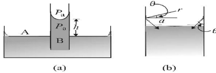
Fig. 11.21 Capillary rise, (a) Schematic picture of a narrow tube immersed in water. (b) Enlarged picture near the interface.
