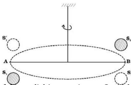
Fig. 9.6 Schematic drawing of Cavendish's experiment. S_1 and S_2 are large spheres which are kept on either side (shown shades) of the masses at A or B. When the big spheres are taken to the other side of the masses (shown by dotted circles), the bar AB rotates a little since the torque reverses direction. The angle of rotation can be measured experimentally.
