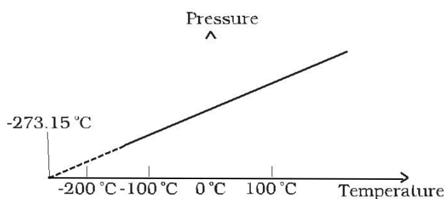
Fig. 12.2 Pressure versus temperature of a low density gas kept at constant volume
