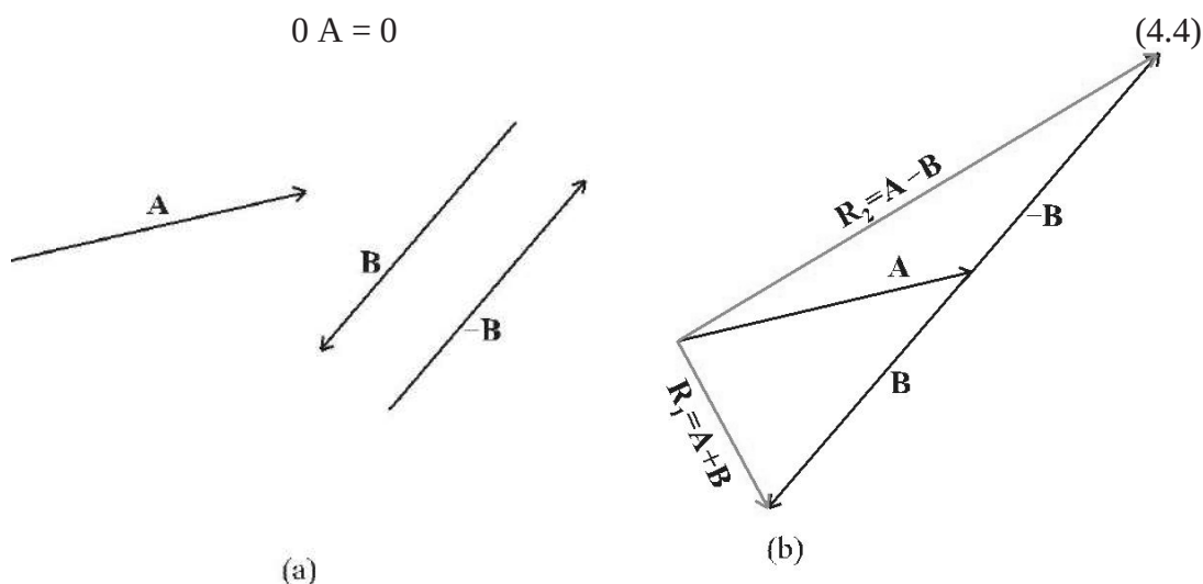
Fig. 4.5 (a) Two vectors A and B , -\mathbf{B} is also shown. (b) Subtracting vector B from vector A —the result is \mathbf{R}_2 . For comparison, addition of vectors A and B , i.e. \mathbf{R}_1 is also shown
