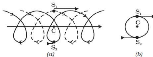
Fig. 7.14 (a) Trajectories of two stars, S_1 (dotted line) and S_2 (solid line) forming a binary system with their centre of mass C in uniform motion. (b) The same binary system, with the centre of mass C at rest.
